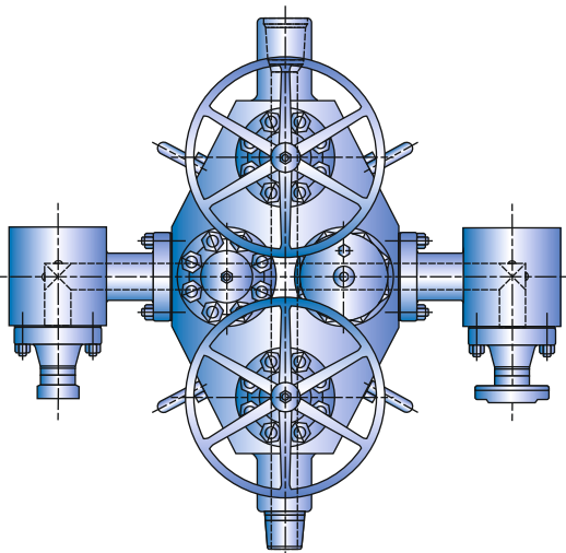
Unitized Well Control Head
