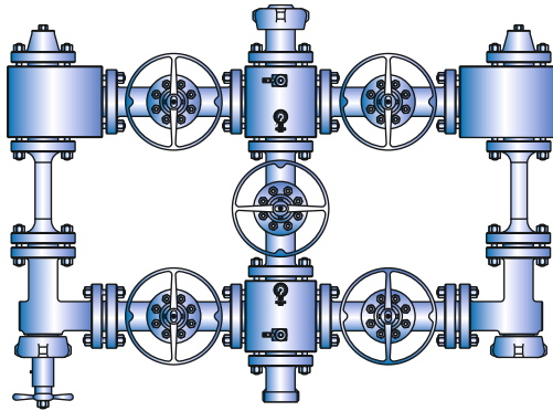
Choke Manifold
