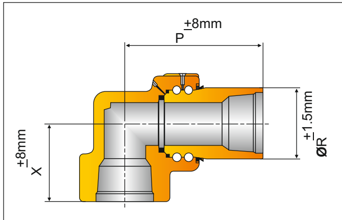
STYLE - 30 SHORT SWEEP SWIVEL JOINT
