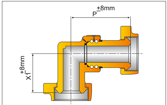
STYLE - 30 SHORT SWEEP SWIVEL JOINT
