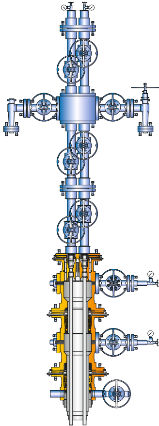
Dual Completion
