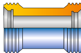
Double Thread (Female)
