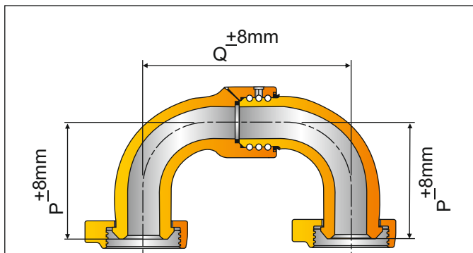
STYLE - 40 LONG SWEEP SWIVEL JOINT END CONNECTION = UNION (M X M) FIG.602/1002/1502* MODEL:- PLSSJ - 40MM
