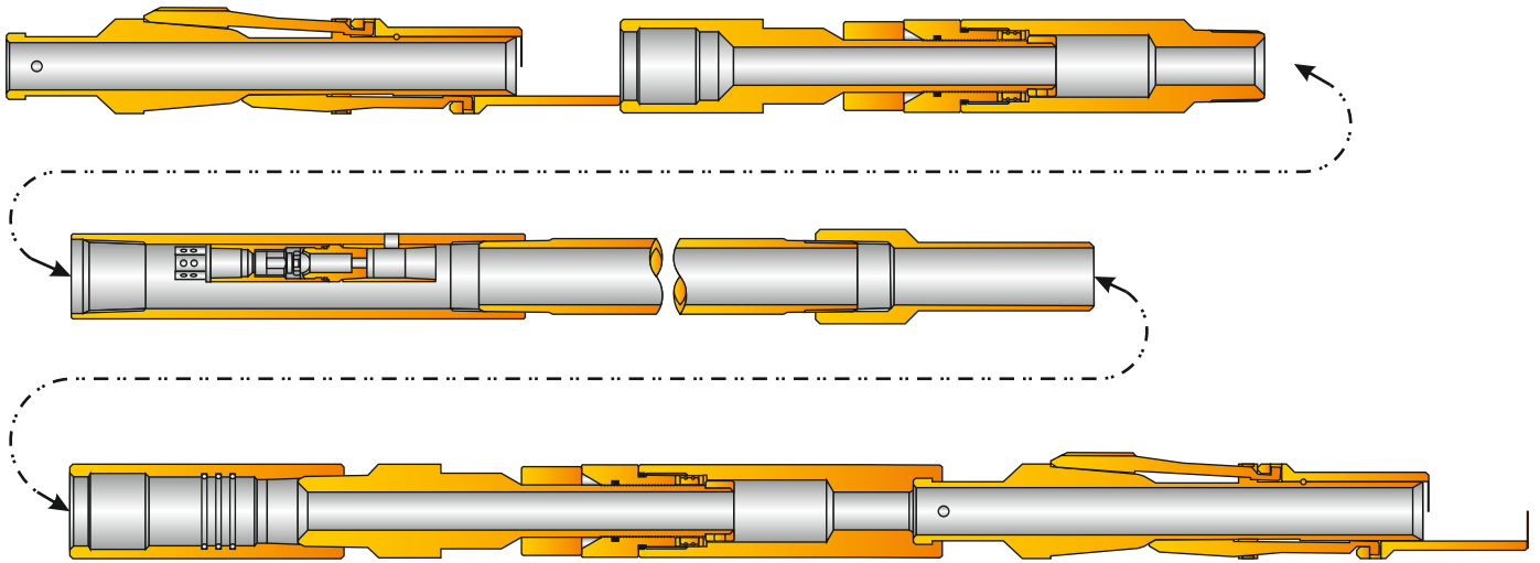
PARVEEN TUBING PACK-OFF ANCHOR ASSEMBLY - 5,000 psi
