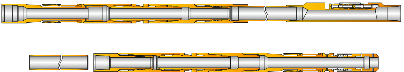
PARVEEN TUBING PACK-OFF ANCHOR ASSEMBLY - 10,000 psi
